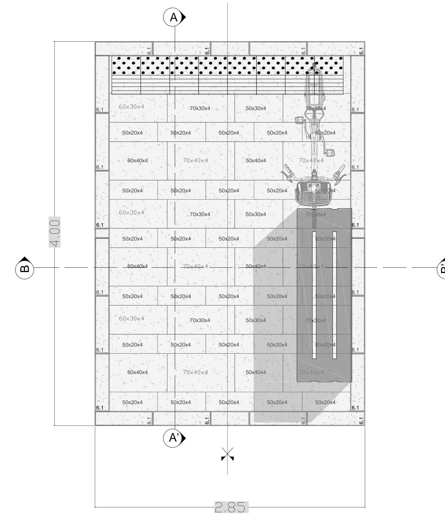
Pocket space - scala 1:100
